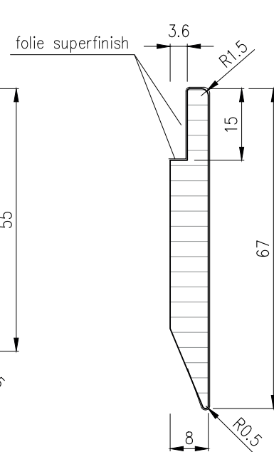
vkladka pro LED 6708
